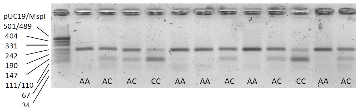
Figure 1. The electrophoretic fractionation in 2% agarose gel of the human DNA amplified PCR and hydrolyzed by endonuclease Apal: first marker-band- pUC19/MspI , 2-13 marker-bands - DNA of the subjects.
